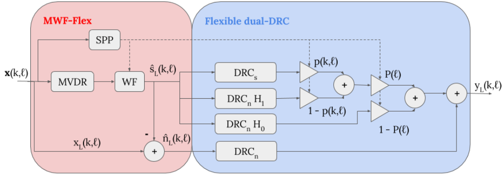
Fig. 2. Schematic overview of the proposed algorithm.
