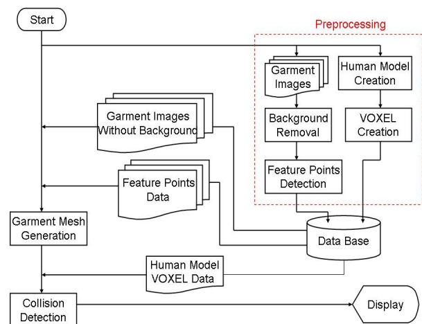
Fig. 1 The processing flow of reconstructing 3D garment mesh by inputting 2D photos. The red dotted rectangle represents the preprocessing stage.
