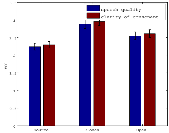
Fig. 8. Results of MOS test on speech quality and clearness of consonants
