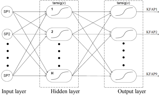
Fig.5. Mapping model between SP and KFAP.
