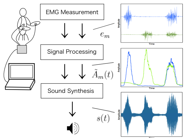
Fig. 1. Proposed sonification system overview.
