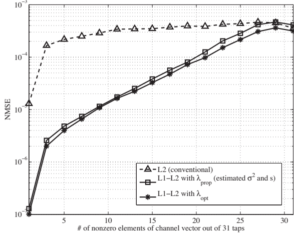
Fig. 6. NMSE versus sparsity (channel order: known)
