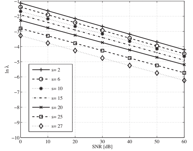
Fig. 4. Optimum values of \lambda versus SNR for different sparsities
