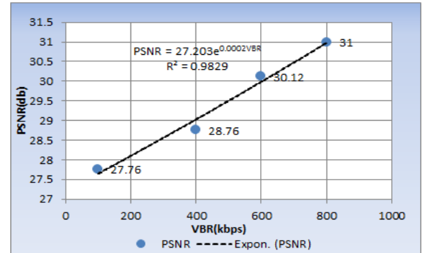
Figure 12. PSNR and Video Bit rate.
