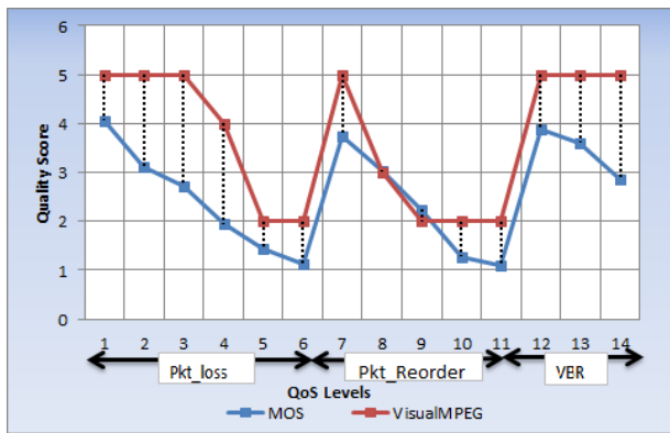
Figure 14. VisualMPEG and PVQ scores across al 14 conditions (see Table V for a description of each degradation condition)
