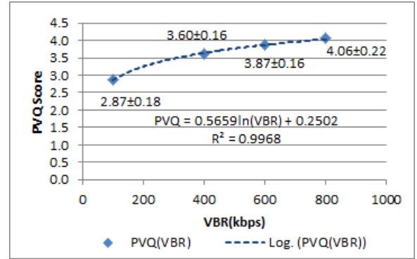
Figure 5. Scatter plot of PVQ ratings vs. Video Bit Rate
