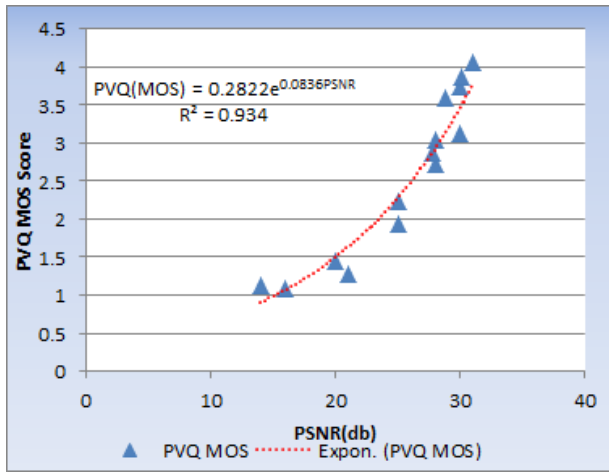
Figure 13. Scatter plot of PSNR vs. PVQ score
