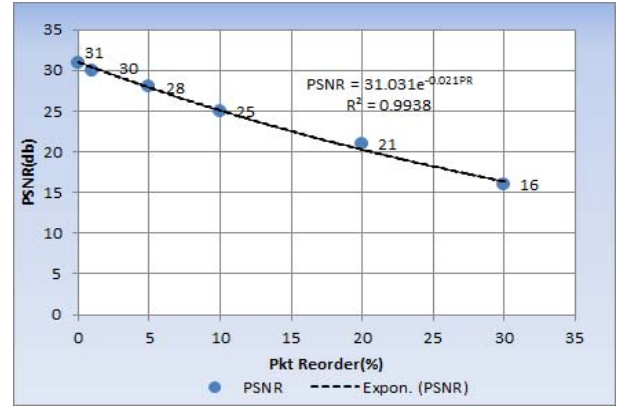
Figure 11. PSNR and Packet Reorder relationship
