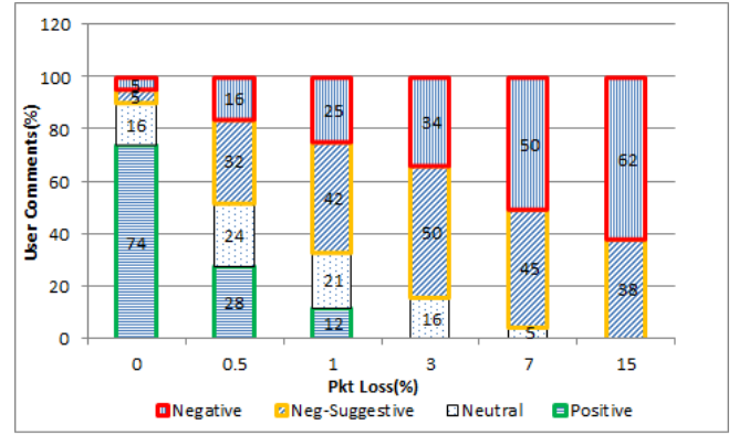
Figure 7. User Comment histogram as a function of PLR
