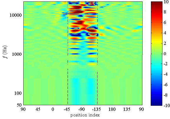
(b) Proposed approach applied to incomplete data
