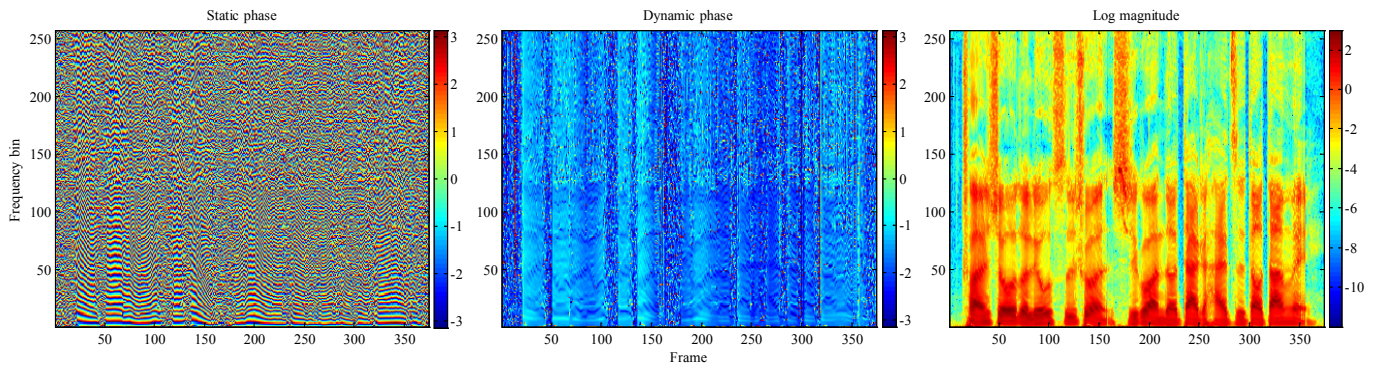
Fig. 4. Static and dynamic phase spectrum as well as their corresponding magnitude spectrum.
