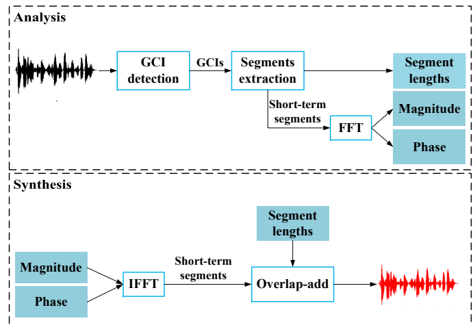
Fig. 1. Our proposed waveform representation framework.
