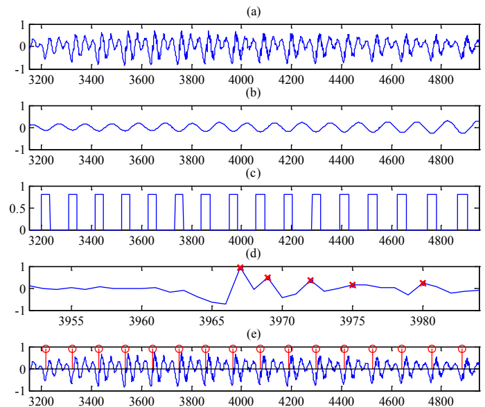
Fig. 2. (a) A section of voiced waveform; (b) The corresponding moving average signal; (c) Short intervals in the moving average signal; (d) LPC residual signal in one interval with candidates marked with red cross; (e) The final GCI locations marked with red stem.
